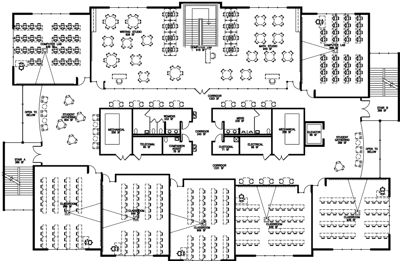
CONSTRUCT NEW MIDTOWN CENTER SCHEMATIC SECOND FLOOR PLAN NOVEMBER 6, 2012
