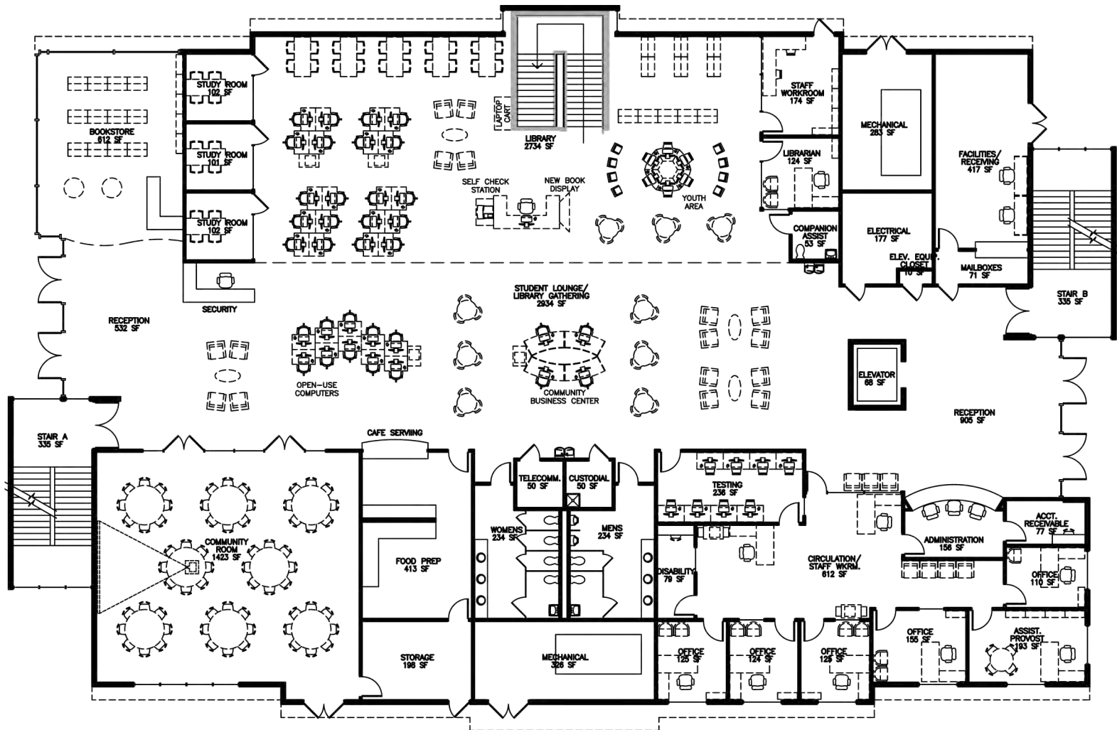
CONSTRUCT NEW MIDTOWN CENTER SCHEMATIC FIRST FLOOR PLAN NOVEMBER 6, 2012
